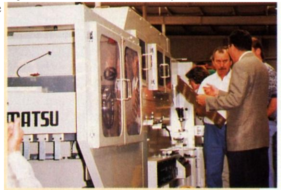
The Marumatsu SuperMax flatbed diecutter from Hitek Equipment can cut and strip with a single die.
